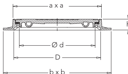
type N 352 NG-R Centerfix 75 mm
