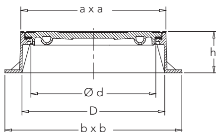
type N 352 NG-R Centerfix 100 - 175 mm
